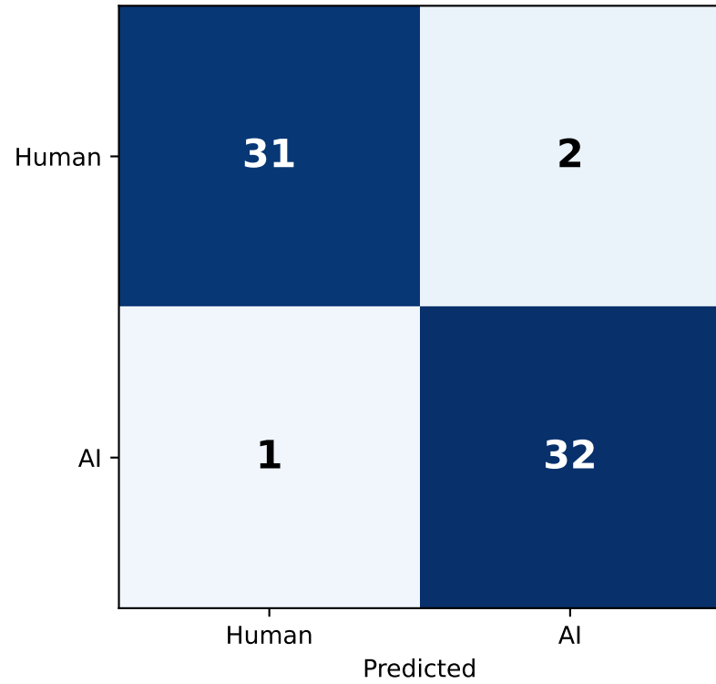
Config A: all 5 features Accuracy: 0.955
