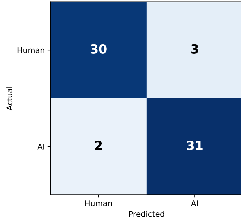
Config B: without LOC Accuracy: 0.924
